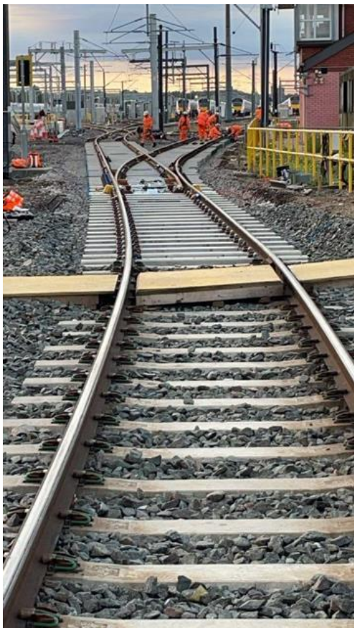
Replacement of 'scissors' points (former access to Hendon Waste Transfer Station siding)
